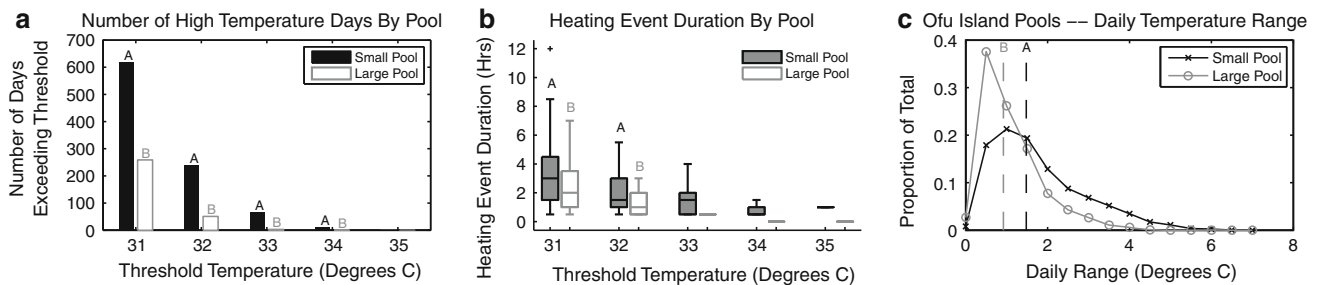
Fig. 3 Thermal Regime of Ofu's Lagoon Pools. a Numbers of days in which in situ temperatures exceeded a given threshold value by pool. Letters indicate a significant distinction between pools (Fisher's exact test, Bonferroni corrected for 5 comparisons, \alpha = 0.01 ). b Distributions of heating event duration above a given thermal
